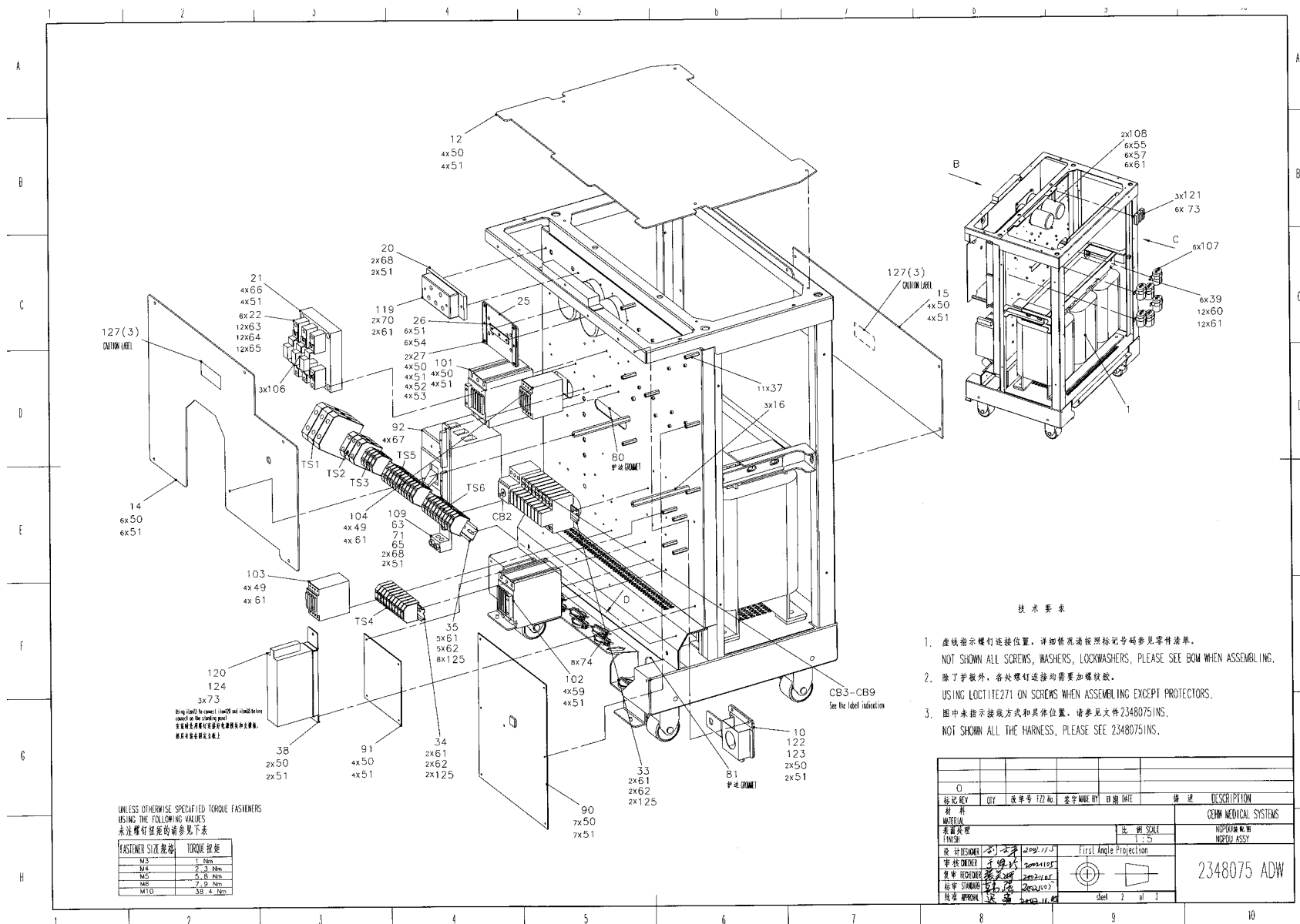
Figure 3-5 NGPDU Assembly2 (2348075, sheet 2, rev 0)
